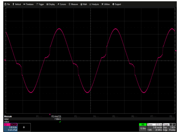
Figure 26: NGB800S48K Input Current Waveform Vin = 115Vac Load: Io = 16.7A Ch 2: I IN
