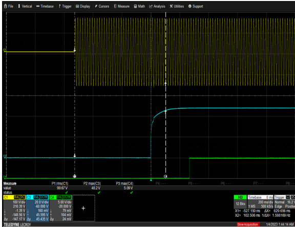
Figure 23: NGB800S48K Turn-on Delay Vin = 115Vac Load: Io = 16.7A Ch 1: V IN Ch 3: Vo Ch 4: DCOK
