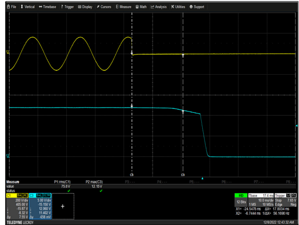
Figure 2: NGB800S12K Hold-up Time Vin = 115Vac Load: Io = 57.5A Ch 1: VIN Ch 3: Vo
