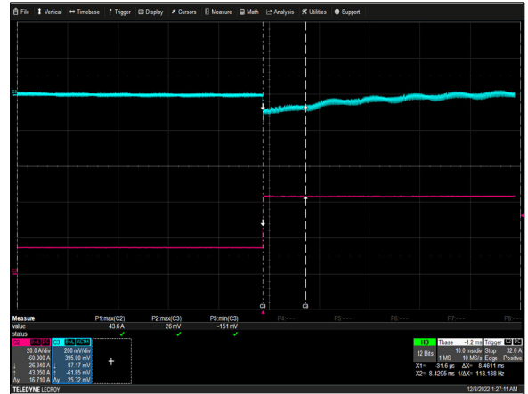
Figure 8: NGB800S12K Transient Response - Vo Deviation Vin = 115Vac Load: Io = 25% to 75%, 0.2A/μs slew rate Ch 2: Io Ch 3: Vo
