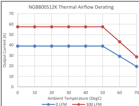
Figure 11: NGB800S12K Derating Curves Vin = 115Vac
