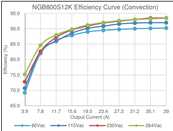
Figure 9: NGB800S12K Efficiency Curve @ 25°C (Convection) Loading: Io_main = 10%Io_max increment to Io_max
