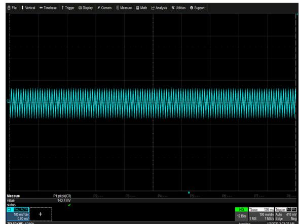
Figure 17: NGB800S24K Ripple and Noise Measurement Vin = 115Vac Load: Io = 33.3A Ch 3: V_o
