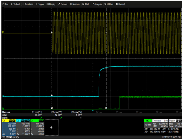
Figure 1: NGB800S12K Turn-on Delay Vin = 115Vac Load: Io = 57.5A Ch 1: VIN Ch 3: Vo Ch 4: DCOCK
