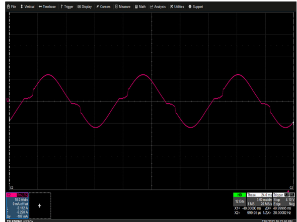
Figure 4: NGB800S12K Input Current Waveform Vin = 115Vac Load: Io = 57.5A Ch 2: IIN
