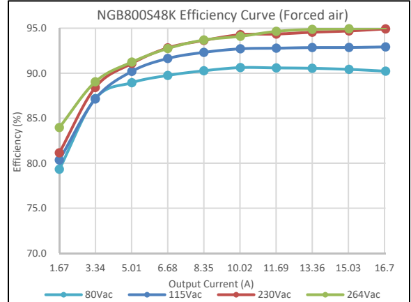
Figure 32: NGB800S48K Efficiency Curve @ 25°C (Forced air) Loading: Io main = 10%Io max increment to Io max
