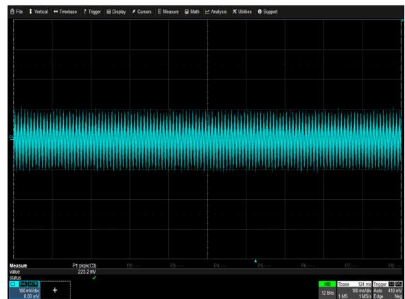
Figure 28: NGB800S48K Ripple and Noise Measurement Vin = 115Vac Load: Io = 16.7A Ch 3: Vo
