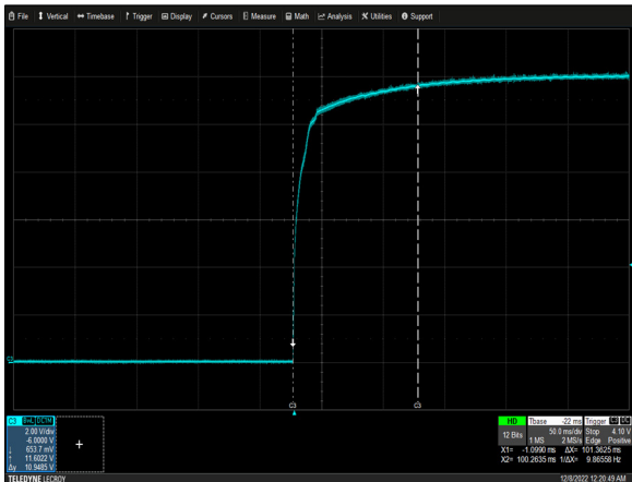
Figure 5: NGB800S12K Output Voltage Startup Characteristic Vin = 115Vac Load: Io = 57.5A Ch 3: Vo
