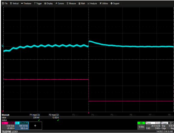
Figure 29: NGB800S48K Transient Response - Vo Deviation Vin = 115Vac Load: Io = 75% to 25%, 0.2A/ \mu s slew rate Ch 2: Io Ch 3: Vo
