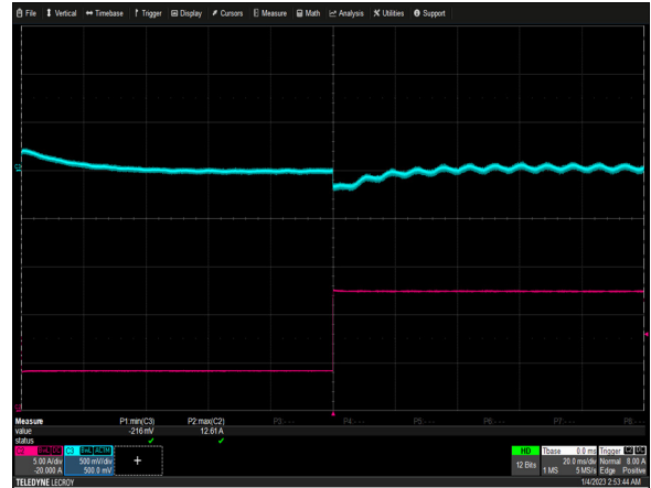
Figure 30: NGB800S48K Transient Response - Vo Deviation Vin = 115Vac Load: Io = 25% to 75%, 0.2A/ \mu s slew rate Ch 2: Io Ch 3: Vo
