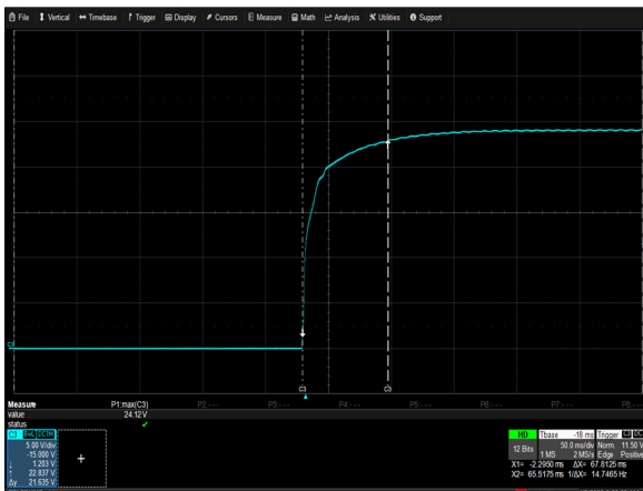
Figure 16: NGB800S24K Output Voltage Startup Characteristic Vin = 115Vac Load: Io = 33.3A Ch 3: V_o
