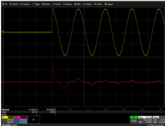
Figure 3: NGB800S12K Inrush Current Vin = 264Vac Load: Io = 0A, Turn on at 90 deg Ch 1: VIN Ch 2: IIN
