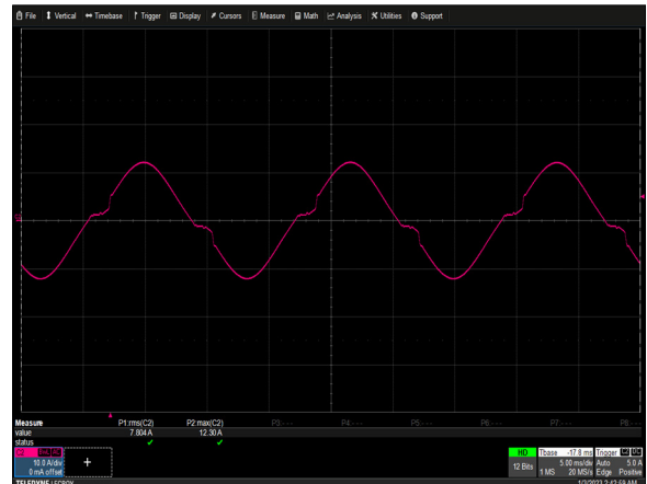
Figure 15: NGB800S24K Input Current Waveform Vin = 115Vac Load: Io = 33.3A Ch 2: I_{IN}
