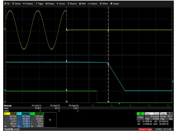
Figure 24: NGB800S48K Hold-up Time Vin = 115Vac Load: Io = 16.7A Ch 1: V IN Ch 3: Vo Ch 4: DCOK
