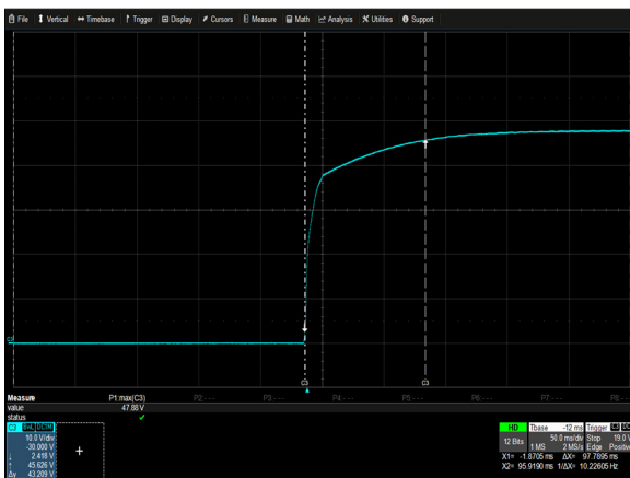
Figure 27: NGB800S48K Output Voltage Startup Characteristic Vin = 115Vac Load: Io = 16.7A Ch 3: Vo
