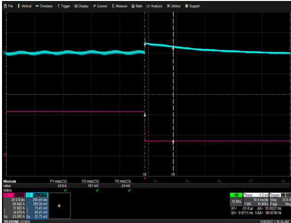
Figure 7: NGB800S12K Transient Response - Vo Deviation Vin = 115Vac Load: Io = 75% to 25%, 0.2A/μs slew rate Ch 2: Io Ch 3: Vo
