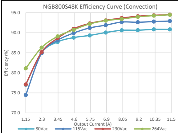
Figure 31: NGB800S48K Efficiency Curve @ 25°C (Convection) Loading: Io main = 10%Io max increment to Io max
