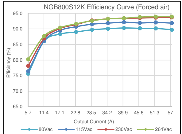
Figure 10: NGB800S12K Efficiency Curve @ 25°C (Forced air) Loading: Io_main = 10%Io_max increment to Io_max
