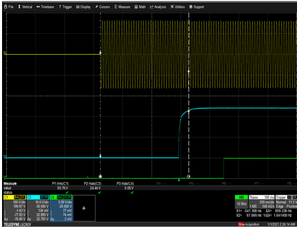
Figure 12: NGB800S24K Turn-on Delay Vin = 115Vac Load: Io = 33.3A Ch 1: V_{IN} Ch 3: V_o Ch 4: DCO
