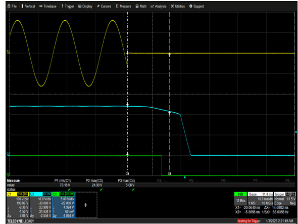
Figure 13: NGB800S24K Hold-up Time Vin = 115Vac Load: Io = 33.3A Ch 1: V_{IN} Ch 3: V_o Ch 4: DCO
